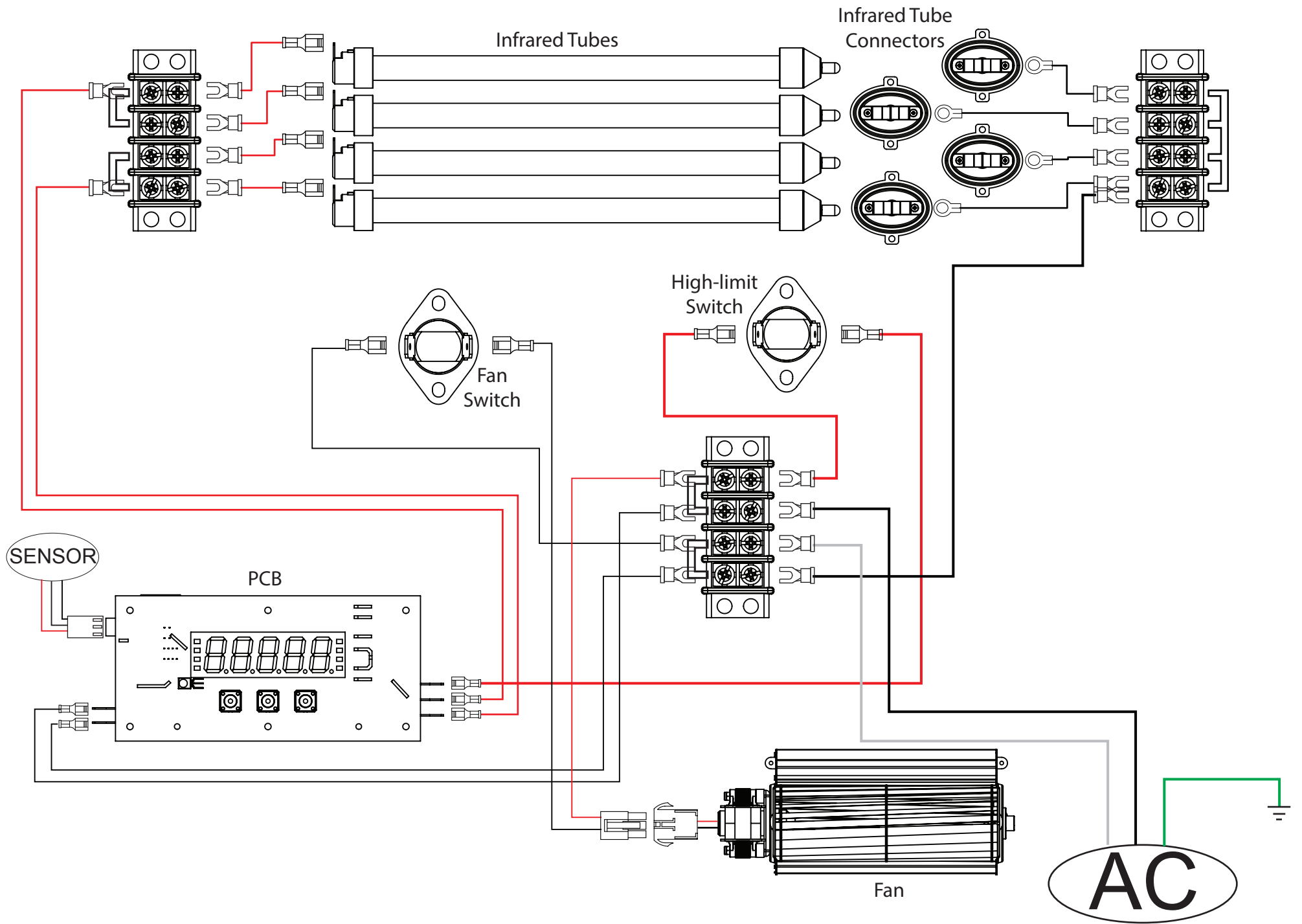
Schematic Bio-1500PB
