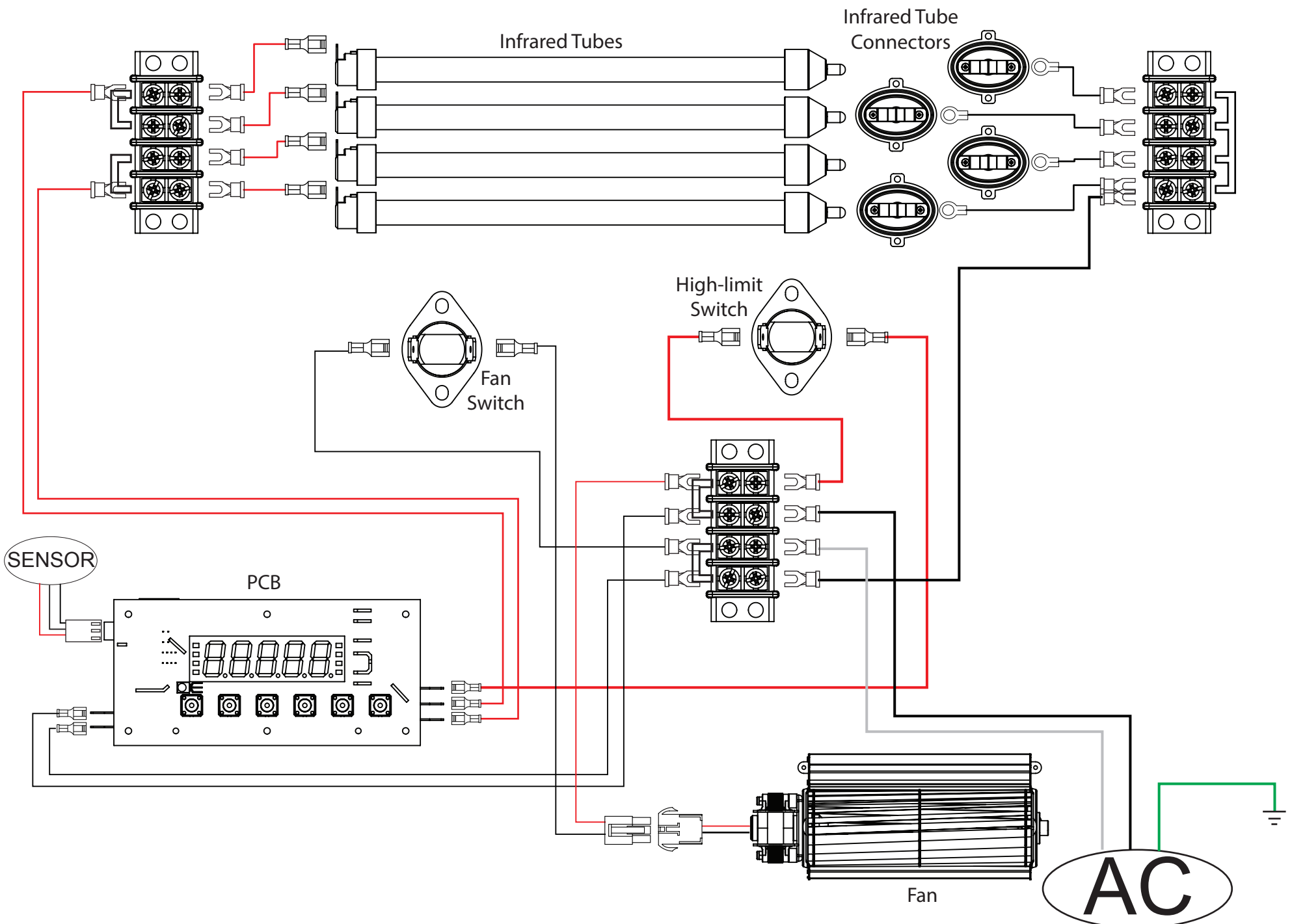
Schematic Bio-1500PCB
