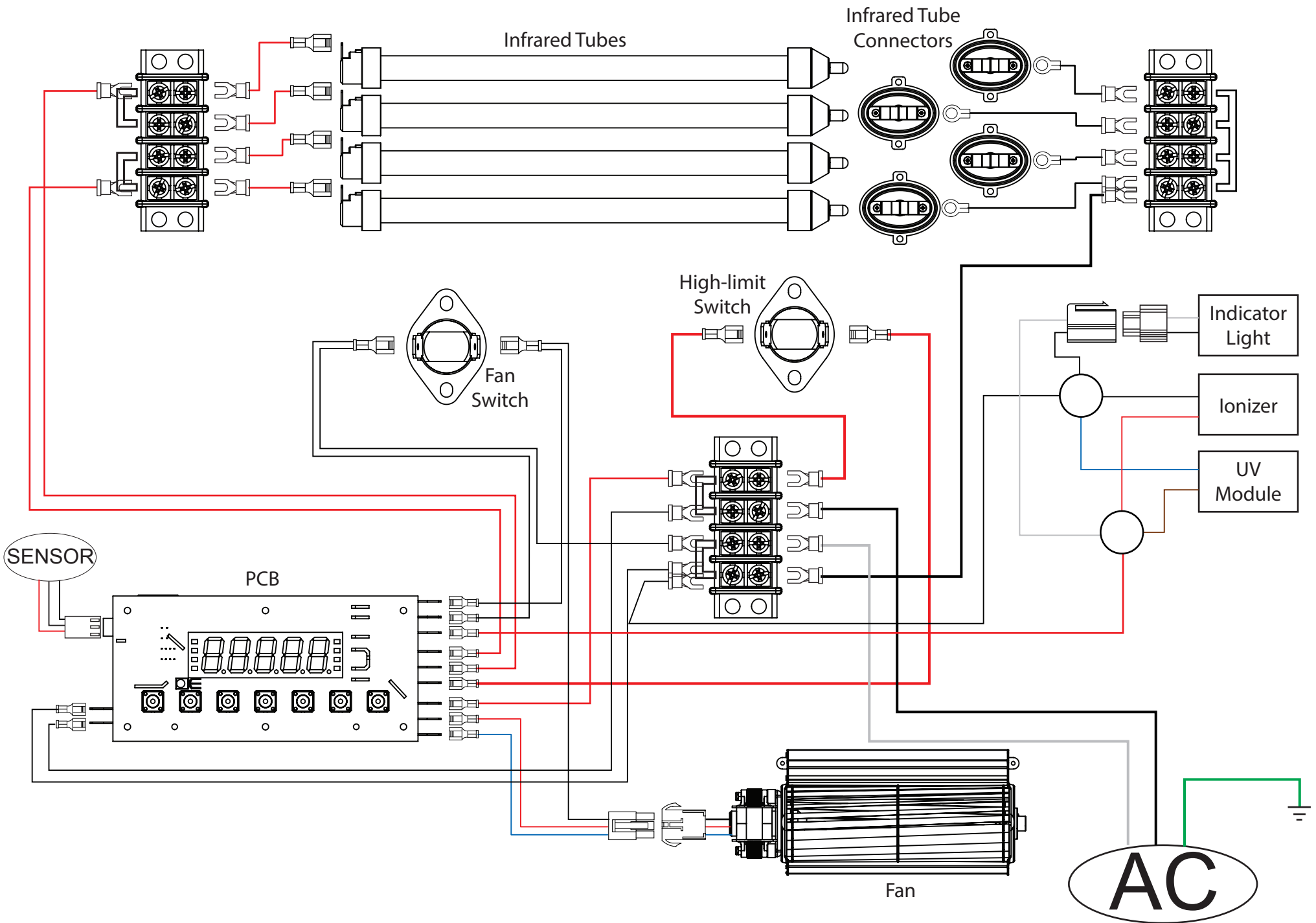
Bio-1500PA with Air-Purification
